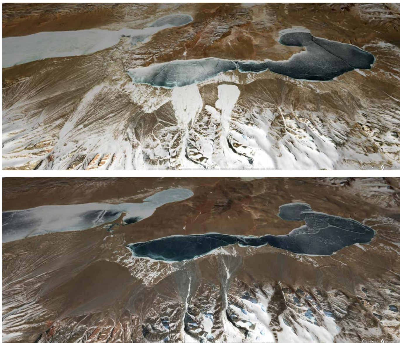
Paired satellite images (from Sentinel-2 true-color) showing the disappearance of glaciers in the Aru Range, Western Tibetan Plateau, China, between 2017 (top) and 2025 (bottom), primarily driven by climate change and warmer temperatures.
